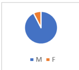
Upper Quartile
