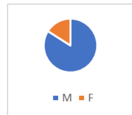
Lower Quartile
